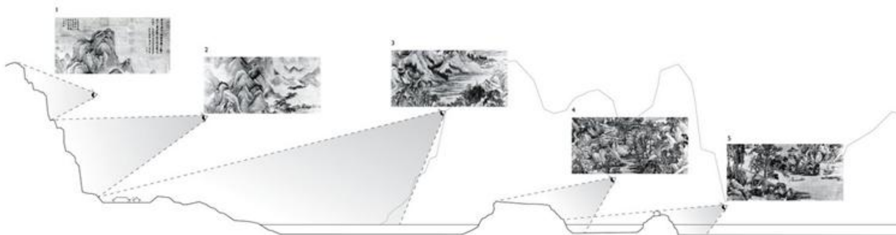
2.15 The five angles of view in Countless Peaks and Valleys
